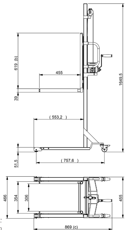
Dimensional Drawing: fixed polyamide rollers version
