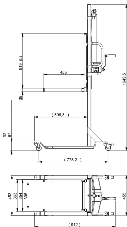
Dimensional Drawing: swivel castor version
